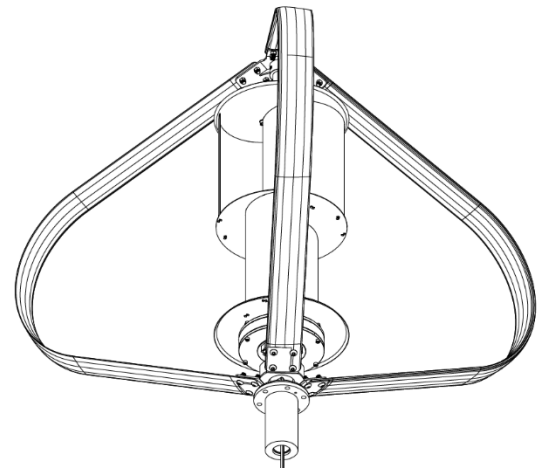
Figure 1: 300 W HI VAWT TECHNOLOGY CORP. Turbine (source: HI VAWT spec sheet S-103-0008)
